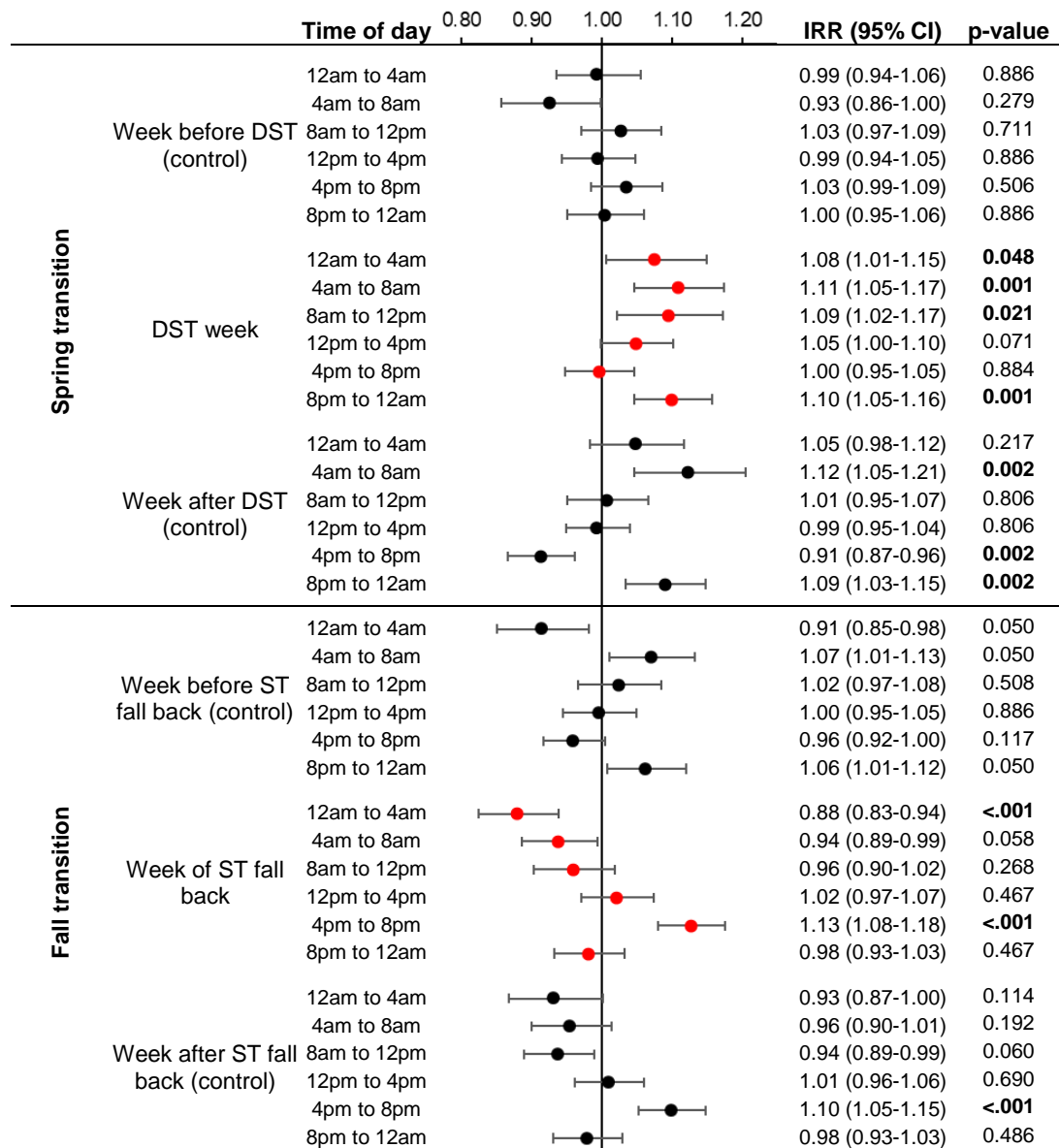
Figure S2: Association of spring DST transition and fall transition back to Standard Time (ST) with fatal MVA risk, stratified by time of day in 4h bins. Related to Figure 2 and Figure 3.
