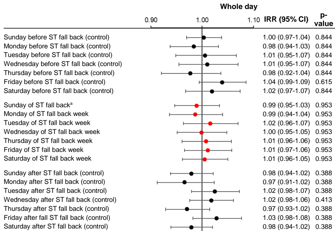
Figure S3: Association of fall transition back to Standard Time (ST) with fatal MVA risk. Weekday effects for the whole day. Related to Figure 3.
