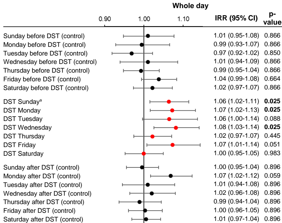
Figure S1. Association of spring DST transition with fatal MVA risk. Weekday effects for the whole day. Related to Figure 2.
